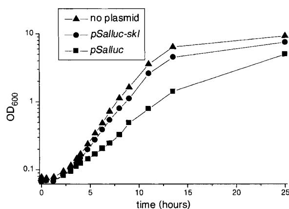
Figure 1. Effect of the peroxisomal luciferase on the growth of the yeast. An overnight culture was diluted to 1 : 100 at time zero and then grown in a shaking incubator at 30 °C, 220 rpm. The control is the BMA64-1A strain without plasmids
