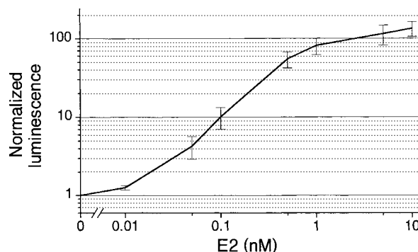
Figure 3. Luciferase activity under oestrogen-inducible promoter. Normalized luminescence measured after 2.5 h incubation in the presence of 17- \beta -oestradiol ( \text{E}_2 ). The curve represents the average of four independent repeats, which were all performed in triplicate. The error bars represent the standard deviation of the four experiments
